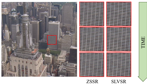
Fig. 3. Temporal domain continuity. We evaluate the performance in three continuous frames. SLVSR is evidently affected less by aliasing.
