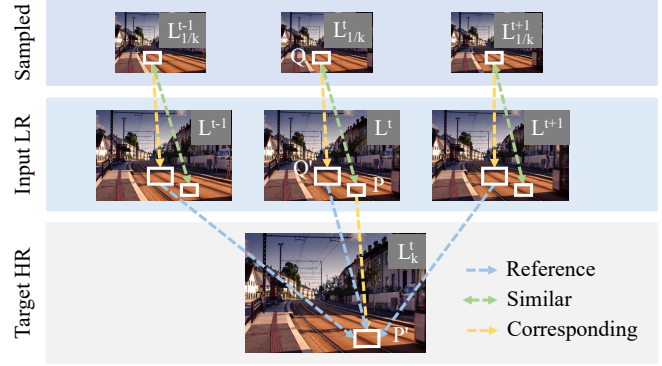
(a) Self-Learned Video Super-Resolution (SLVSR). Sampled images are down-sampled from Input LR images. The definition of the marks is shown in Sec. 2.2.
